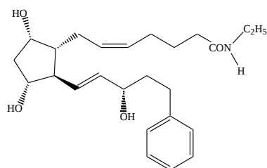
(structure of bimatoprost)
