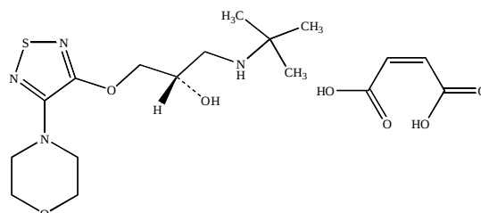
(structure of timolol maleate)
